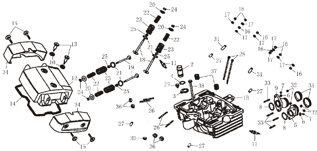
E-1: 气缸盖总成 (Cylinder head assembly)
