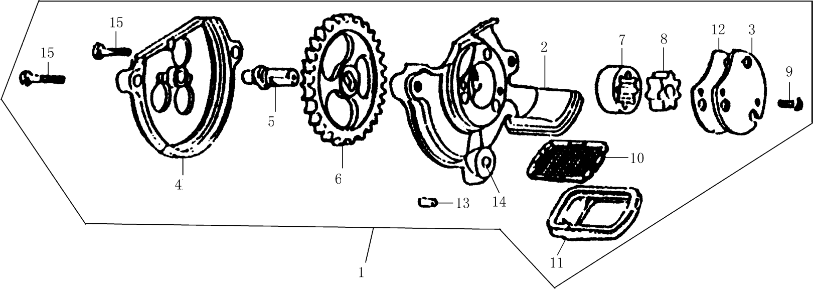
E-6: 机油泵总成 (Oil pump assembly)
