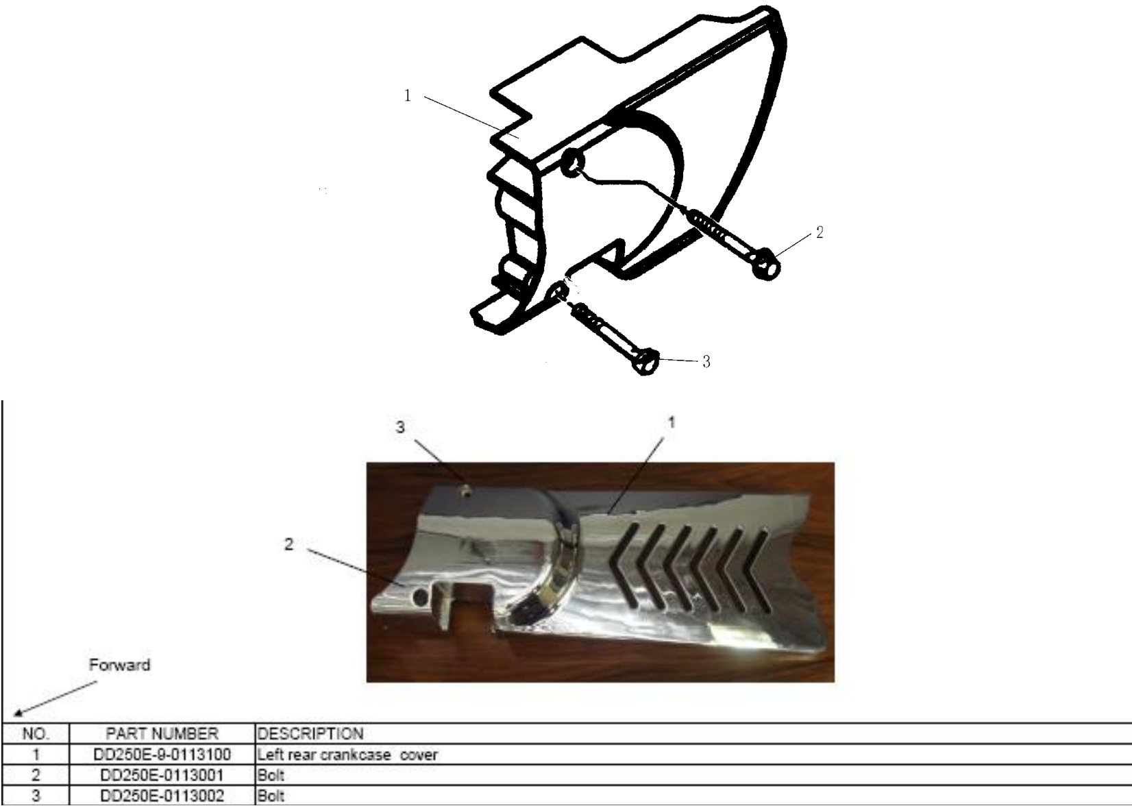
E-13: 左曲轴箱后盖总成(Left rear crankcase cover assembly)
